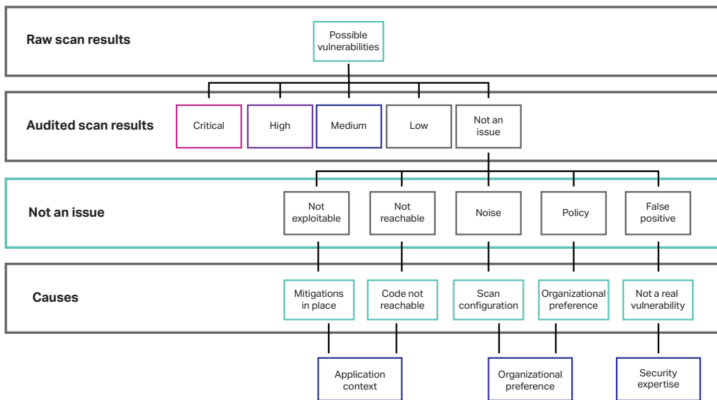
Figure 1. Scan finding classification
