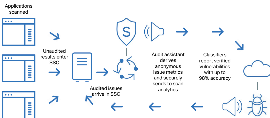
Figure 2. Audit Assistant workflow
